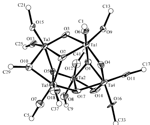
Fig. 3 Structure of compound 4. Details as in Fig. 1.
